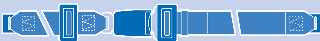
Static lap strap with 90° anchor plates with adjustor built into webbing buckle allowing both ends to be adjusted to suit your application.
